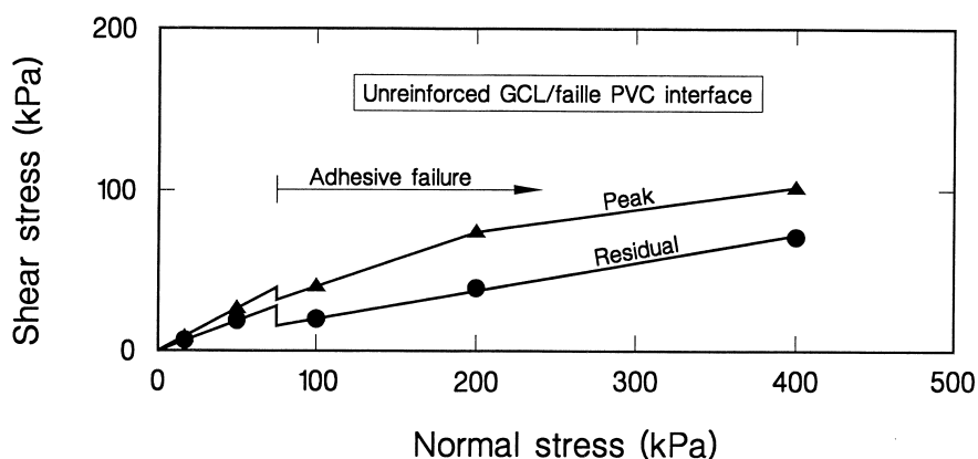
Figure 13. Peak and residual failure envelopes for an unreinforced, smooth HDPE geomembrane-backed GCL-faille PVC geomembrane interface.
