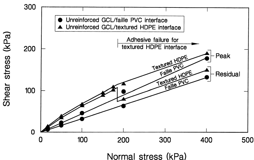
Figure 15. Comparison of failure envelopes for unreinforced, textured HDPE geomembrane-backed GCL-faille PVC and textured HDPE geomembrane interfaces.
