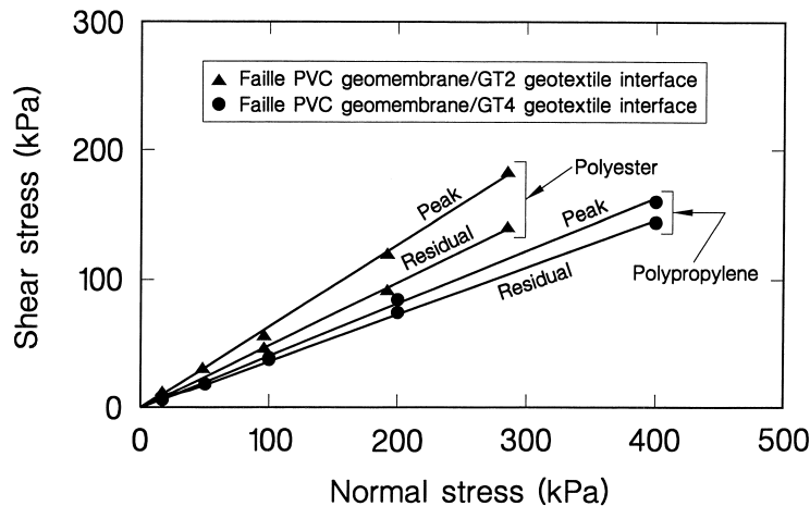
Figure 7. Effect of nonwoven geotextile fiber composition on interface shear strength.
