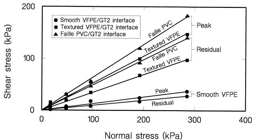
Figure 5. Comparison of failure envelopes for faille PVC, smooth VFPE, and textured VFPE geomembrane-GT2 geotextile interfaces.
