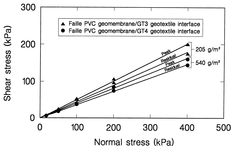
Figure 9. Effect of nonwoven geotextile mass per unit area on interface shear strength.
